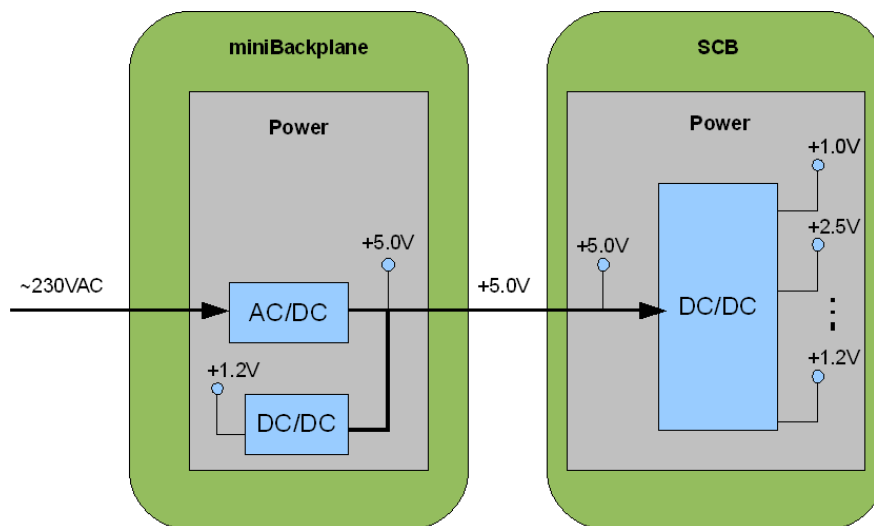
Figure 8: Power supply basic architecture.
