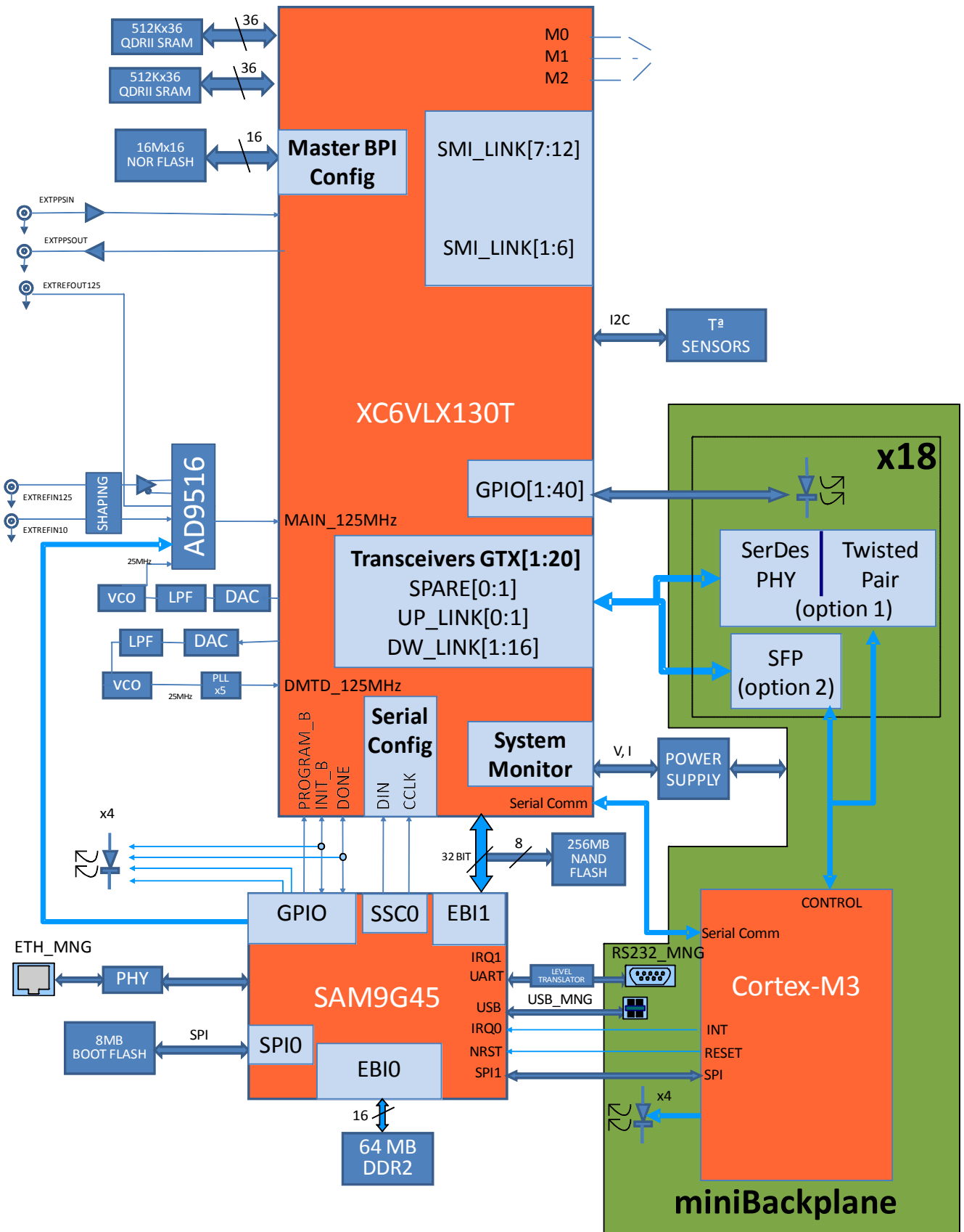
Figure 7: miniBackplane WRS Functional Block Diagram.
