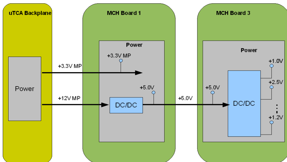
Figure 4: Power supply basic architecture.
