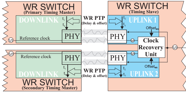
Figure 1: Seamless switch-over.
